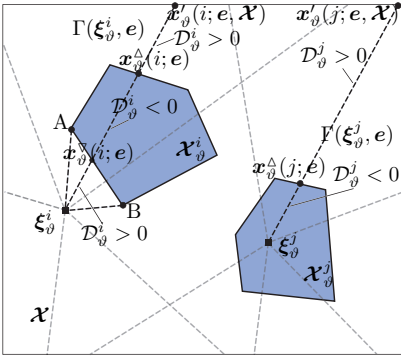
Fig. 3. Point \xi_\vartheta^j belongs to the interior of \mathcal{X}^j , which implies that the intersection of the ray \Gamma(\xi_\vartheta^j, e) with the boundary \text{bd}(\mathcal{X}^j) of the cell \mathcal{X}^j will be a singleton for all e \in \mathbb{S}^1 . On the other hand, point \xi_\vartheta^i does not belong to \mathcal{X}^i , and in this case, the intersection of \Gamma(\xi_\vartheta^i, e) with \text{bd}(\mathcal{X}^i) can 1) be empty, 2) consist of two points or 3) be a single point (vertex of a cell), namely point A or point B.
