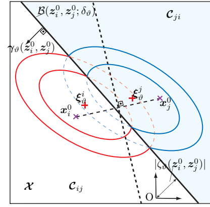
Fig. 2. The projection of the bisector \mathcal{B}(z_i^0, z_j^0; \delta_\vartheta) into \mathcal{X} is a line segment, which is neither (by default) perpendicular to the line segment [x_i^0, x_j^0] (note that the points x_i^0 and x_j^0 are the projections of z_i^0 and z_j^0 into \mathcal{X} , respectively) nor it passes through the midpoint of the same segment, as does the bisector of x_i^0 and x_j^0 in a standard Voronoi partition, which is shown in dashed line. It also corresponds to the collection of all points in \mathcal{X} that belong to the intersections of the c -level sets of \delta_\vartheta(\cdot; z_i^0) and \delta_\vartheta(\cdot; z_j^0) , for all c \geq 0 .
