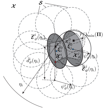
Fig. 4. The i -th agent will increase its communication range until it discovers all of its neighbors in the topology of \mathfrak{V}_\vartheta(\mathcal{Z}^0) (or, equivalently, in the topology of \mathcal{X}_\vartheta(\mathcal{Z}^0) ). To simplify this illustration, we have assumed that \mu_\vartheta^i = \mu_\vartheta^j = 0 , which implies that the ellipsoids \bar{\mathcal{E}}_\vartheta^i(\eta_i) , \bar{\mathcal{E}}_\vartheta^j(\eta_j) and \bar{\mathcal{E}}_\vartheta^i(\eta_i) are all equal modulo a linear translation.
